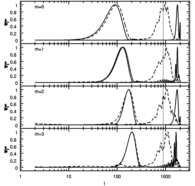
FIG. 10. Effect of measuring only one Stokes parameter on 20% of the pixels chosen at random. The panels show the window functions for the first modes with m=0,1,2,3 when both Stokes parameters are measured (solid lines) and when 20% are missing (dashed lines).
